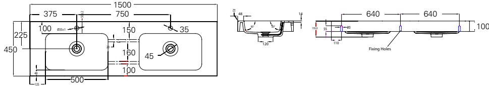
1B3.1314 Splash Basin Top 1500mm Double Bowl
