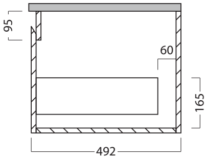
Side Section Showing Bottom Drawer
