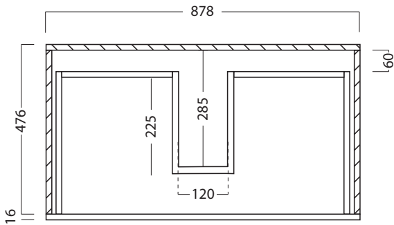
Top Section of Bottom Drawer
