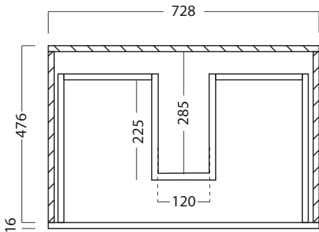
Top Section of Bottom Drawer
