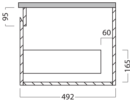
Side Section Showing Bottom Drawer
