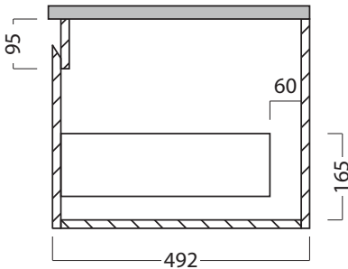
Side Section Showing Bottom Drawer
