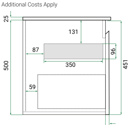
Side Section Showing Add-on Concealed Drawer
