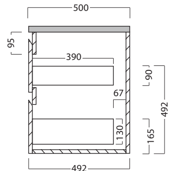
Side Section Showing Bottom Drawer
