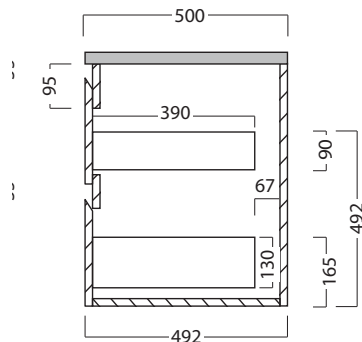
Side Section Showing Bottom Drawer
