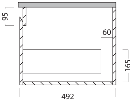
Side Section Showing Bottom Drawer
