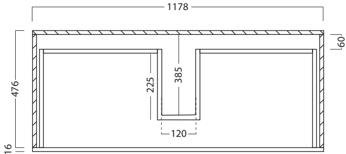
Top Section of Bottom Drawer
