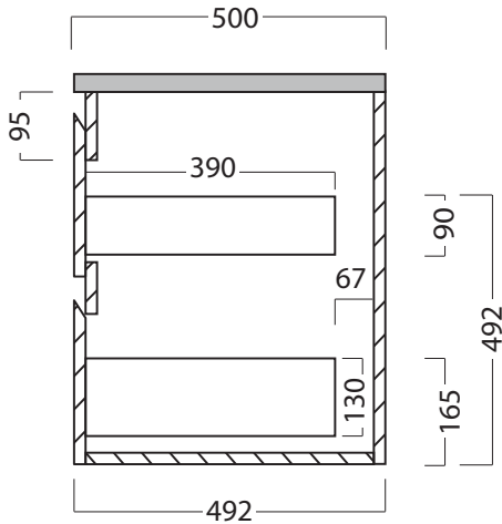
Side Section Showing Bottom Drawer
