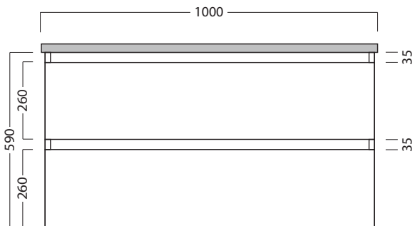
Top Section of Bottom Drawer
