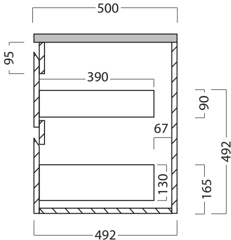
Side Section Showing Bottom Drawer
