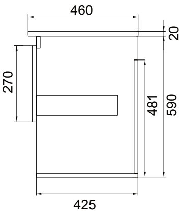
Side Section
