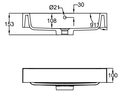
Front Section of Basin
