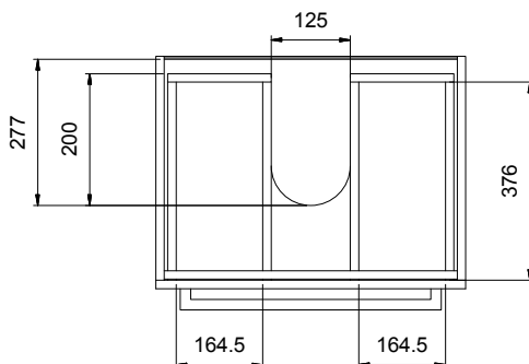
Top Section of Drawer
