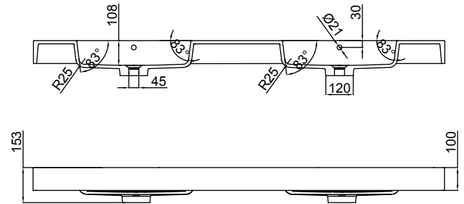
Front Section of Basin
