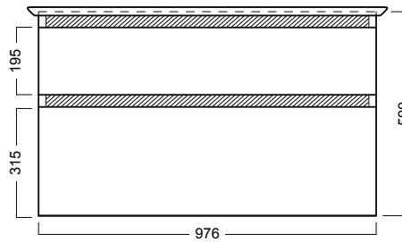
Top Section
