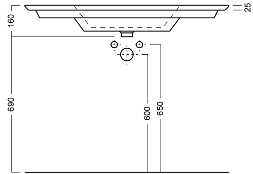
Side Section
