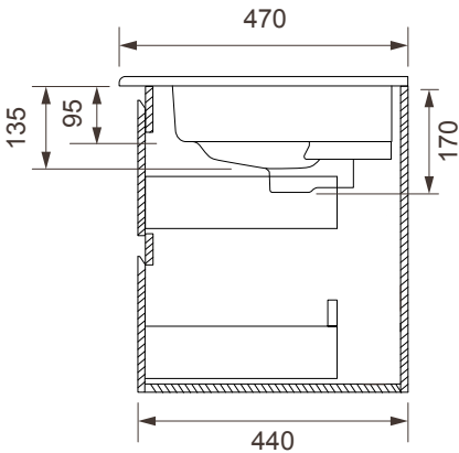
Side Section
