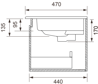
Side Section
