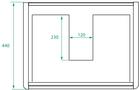
Top Down
