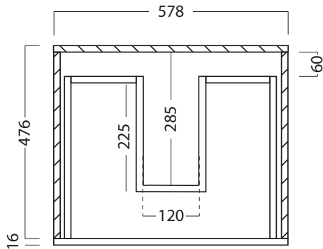
Top Section of Drawer
