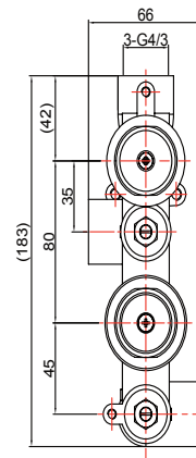
Cross Section Front View
