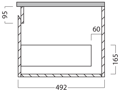
Side Section Showing Add-on Concealed Drawer
