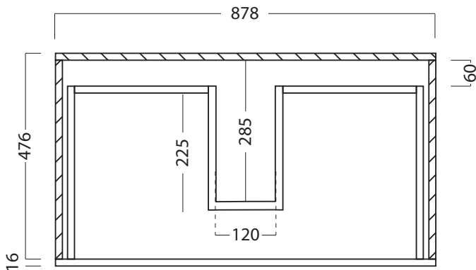
Top Section of Bottom Drawer
