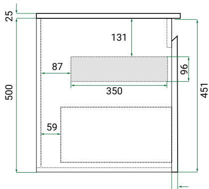
Side Section Showing Add-on Concealed Drawer
