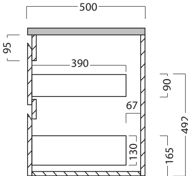
Side Section Showing Bottom Drawer
