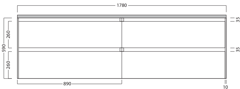
Top Section of Bottom Drawer
