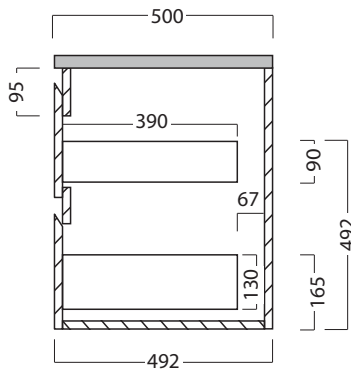
Side Section Showing Bottom Drawer
