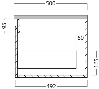
Side Section Showing Bottom Drawer
