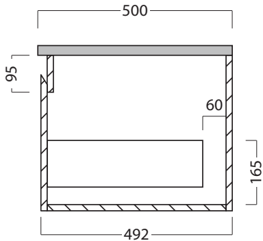
Side Section Showing Bottom Drawer
