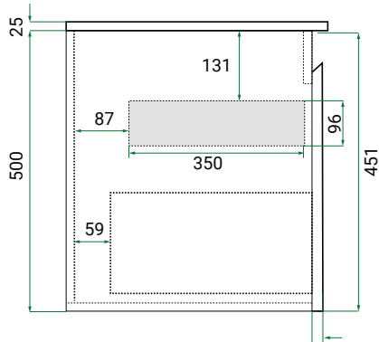
Side Section Showing Add-on Concealed Drawer
