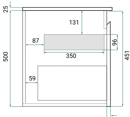
Side Section Showing Add-on Concealed Drawer
