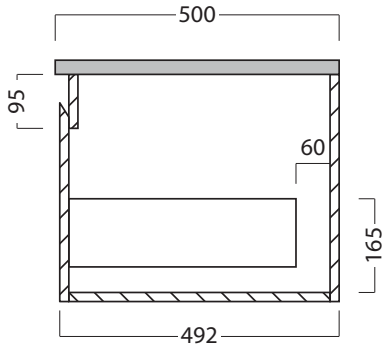
Side Section Showing Bottom Drawer
