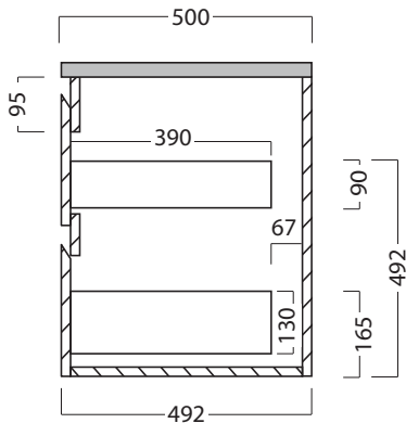
Side Section Showing Bottom Drawer
