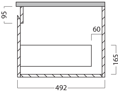
Side Section Showing Bottom Drawer
