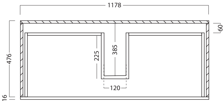
Top Section of Bottom Drawer
