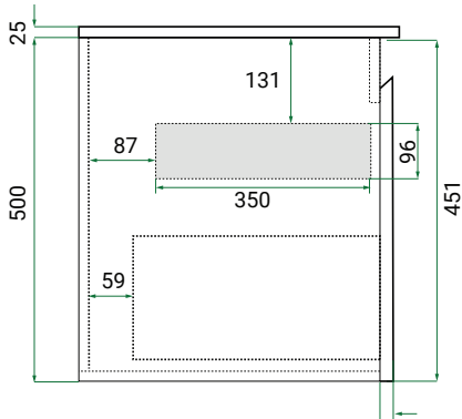
Side Section Showing Add-on Concealed Drawer
