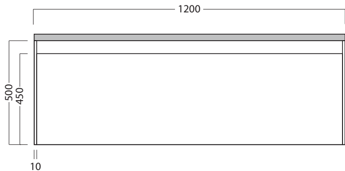
Top Section of Bottom Drawer
