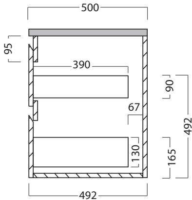
Side Section Showing Bottom Drawer
