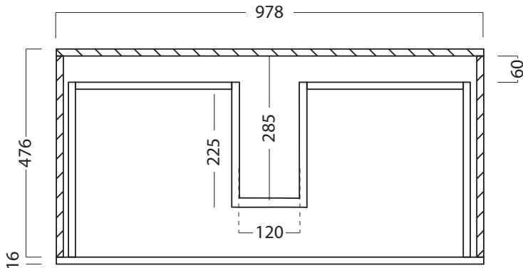
Top Section of Bottom Drawer
