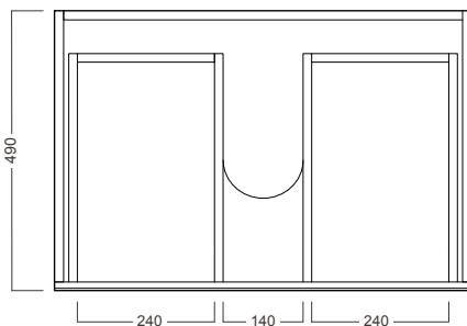
Drawer Cross Section
