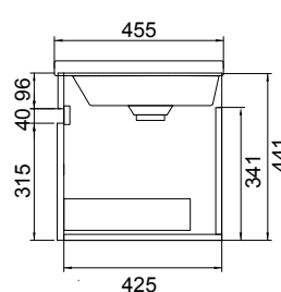
Side Section
