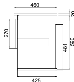
Side Section
