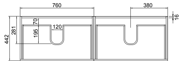
Side Section
