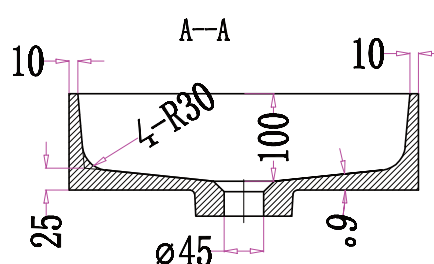
Front Section
