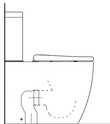
Side Section
