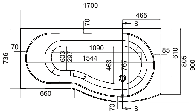
Top Down
