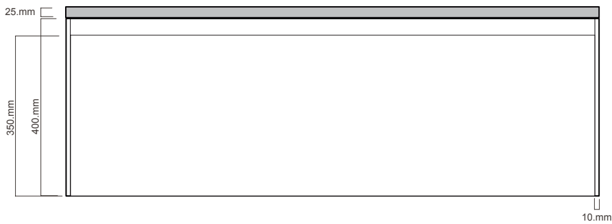
FRONT VIEW
