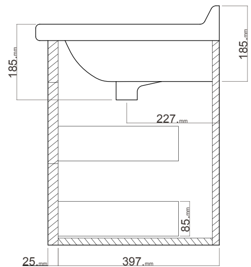
SIDE WASHBASIN
