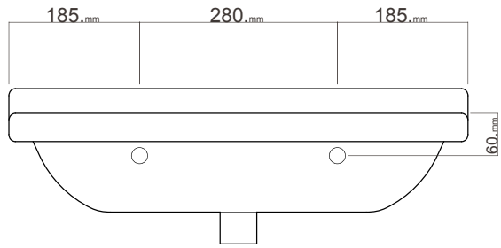
BACK WASHBASIN
