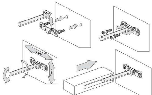
Fixing Mechanism
