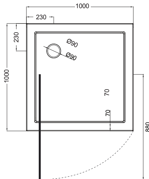
Shower Tray (BSF-1000S)
