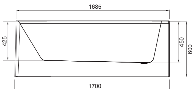
Side Section
